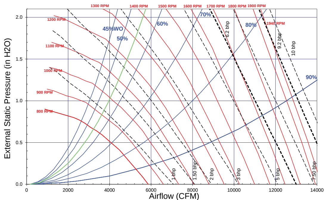
Figure 21. Fan curves - 12.5 ton (high efficiency) to 25 ton, horizontal
