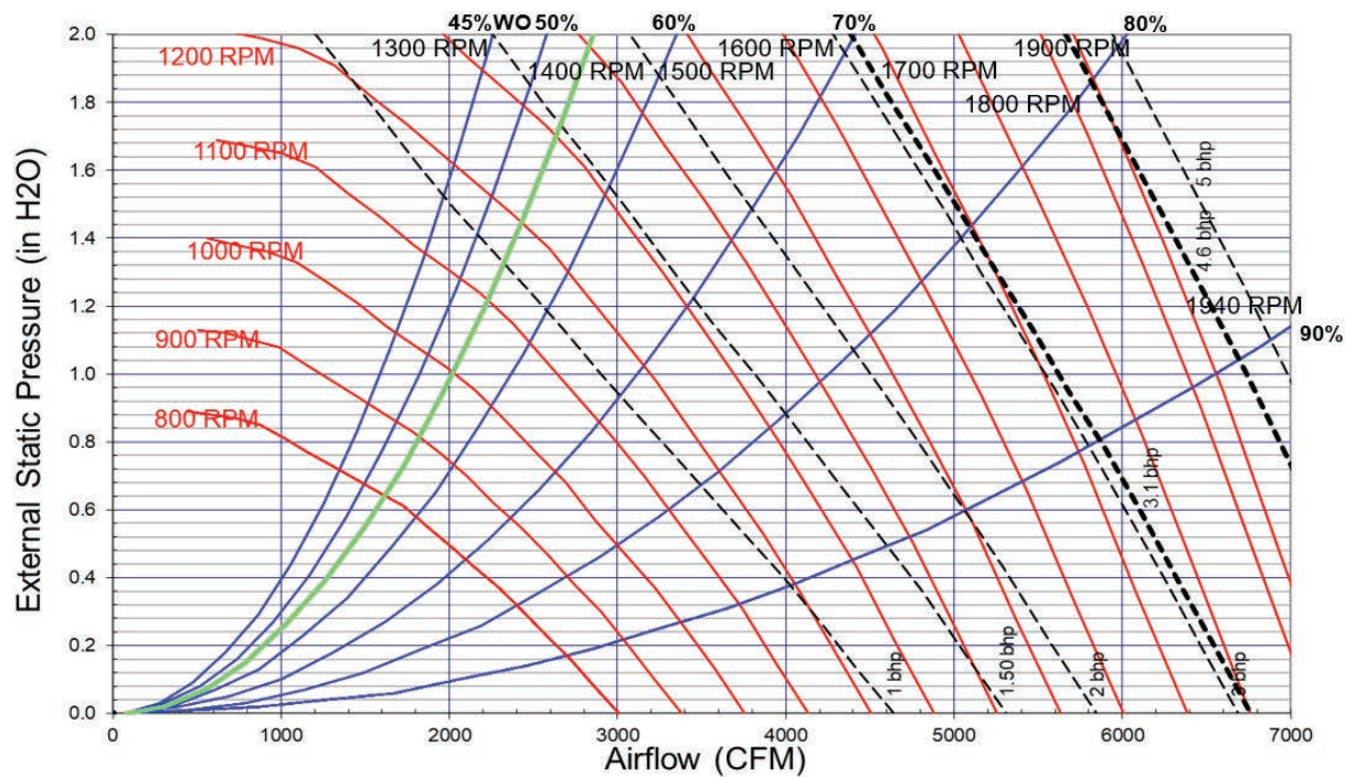
Figure 16. Fan curves — 6 to 10 tons (model T*K), downflow
