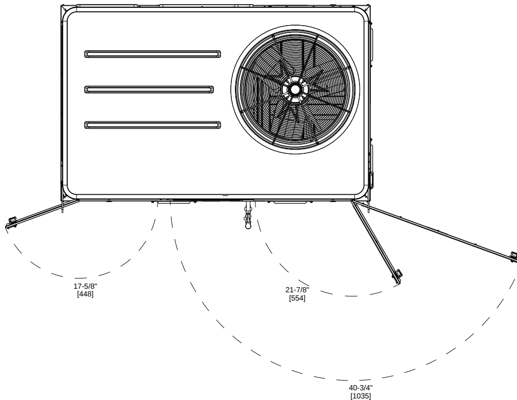
Figure 32. B.0 cabinet
