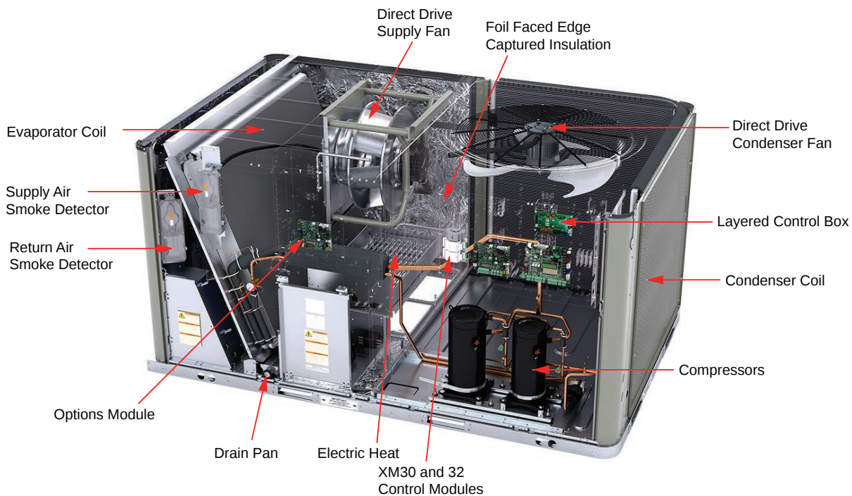
Figure 1. Unit overview
