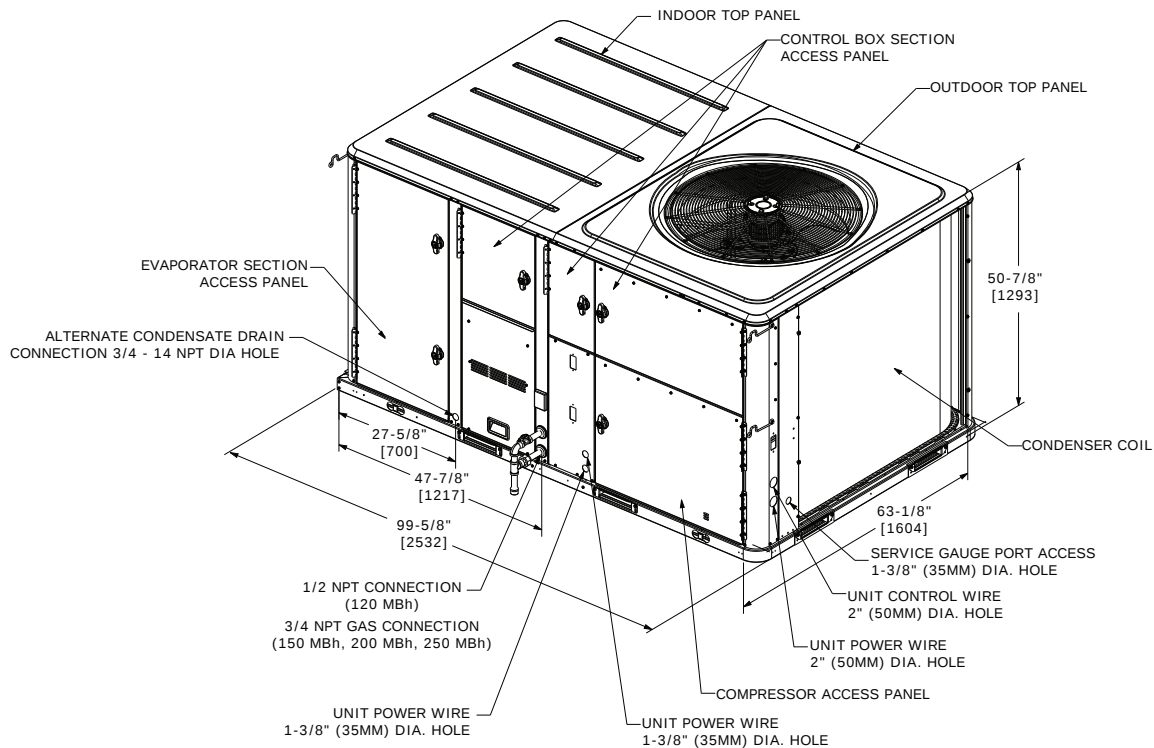
Figure 40. C.0 cabinet – downflow airflow supply/return, through-the-base utilities
