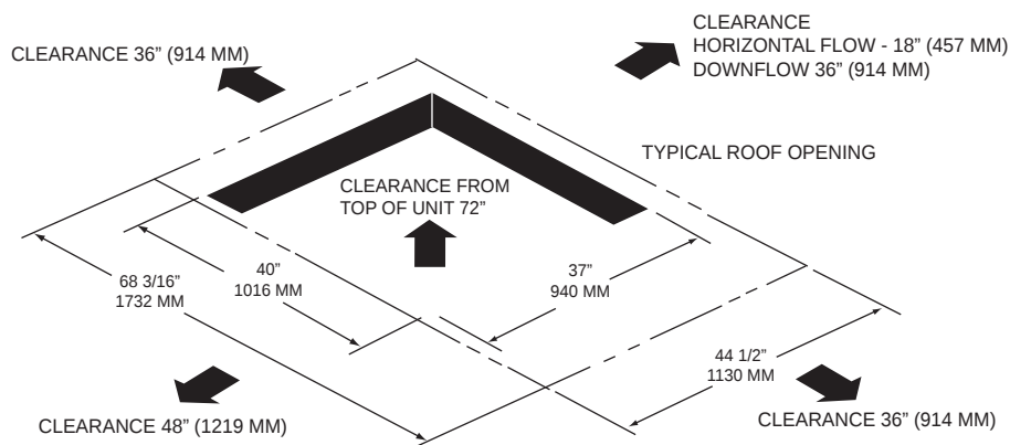
Figure 28. A.0 cabinet – unit clearance and roof opening
