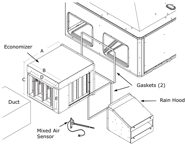
Figure 16. BAYCON207, BAYECON208A horizontal economizer and rain hood
