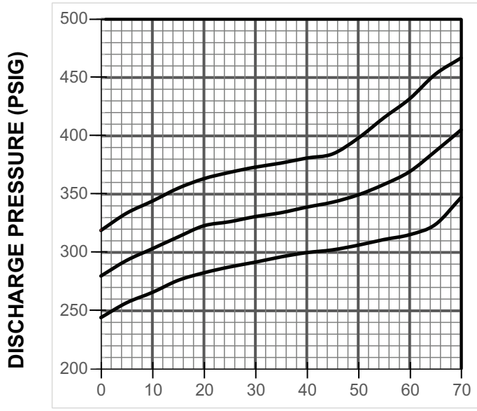
Figure 15. 4 Ton HP (X48 Models)
