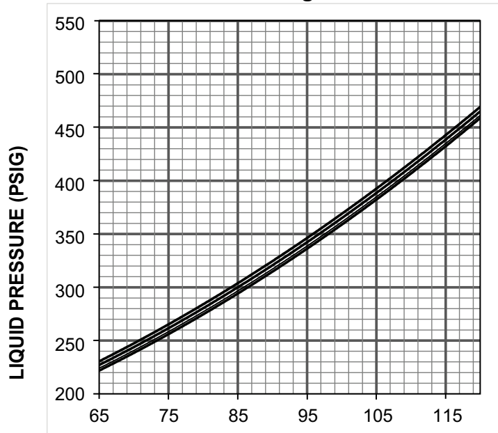
Figure 20. 5 Ton AC (X60 Models)
