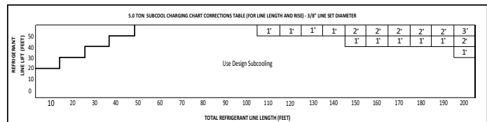
Figure 5. Subcool Charging Corrections – X60 Models (3/8)
