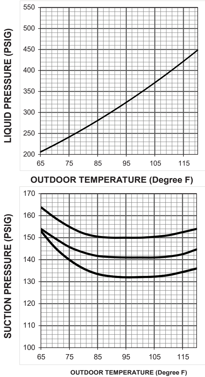
Figure 17. 2 Ton AC (X24 and X25 Models)
