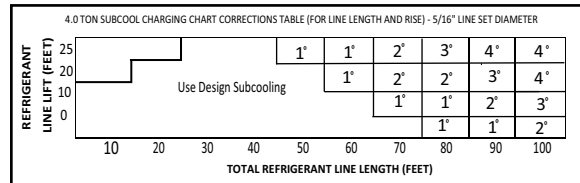
Figure 4. Subcool Charging Corrections – X60 Models (5/16)
