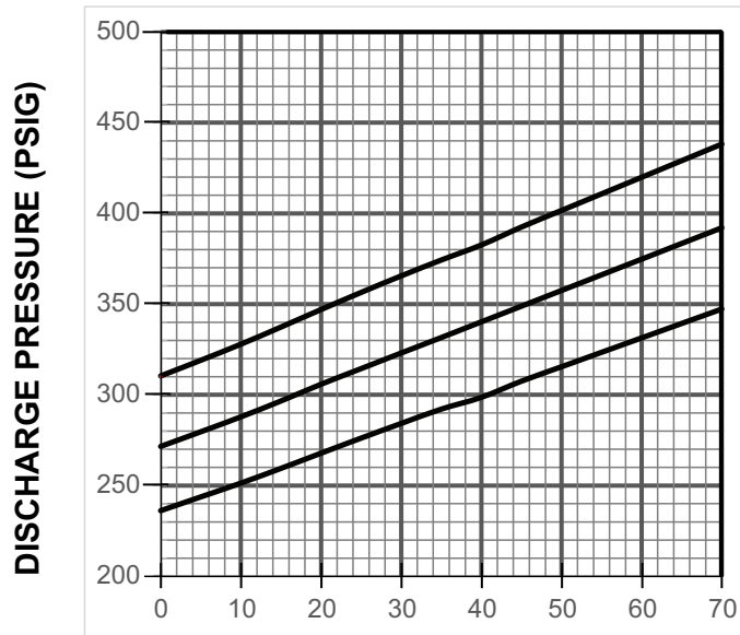
Figure 14. 3 Ton HP (X36 Models)
