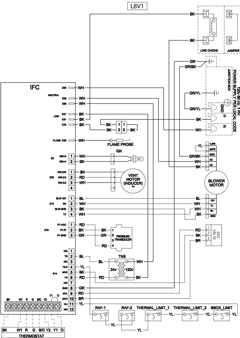
Figure 2. L8V1 – ladder diagram
