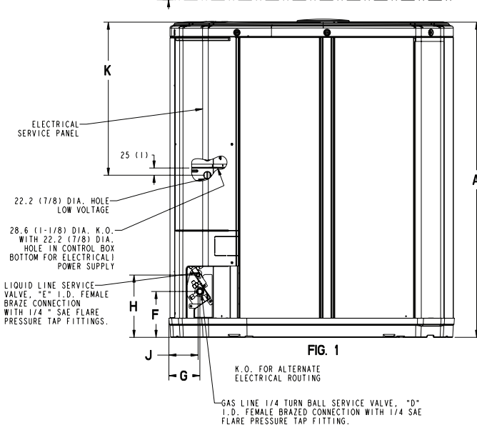
From Dwg. D152862 Rev. 21
